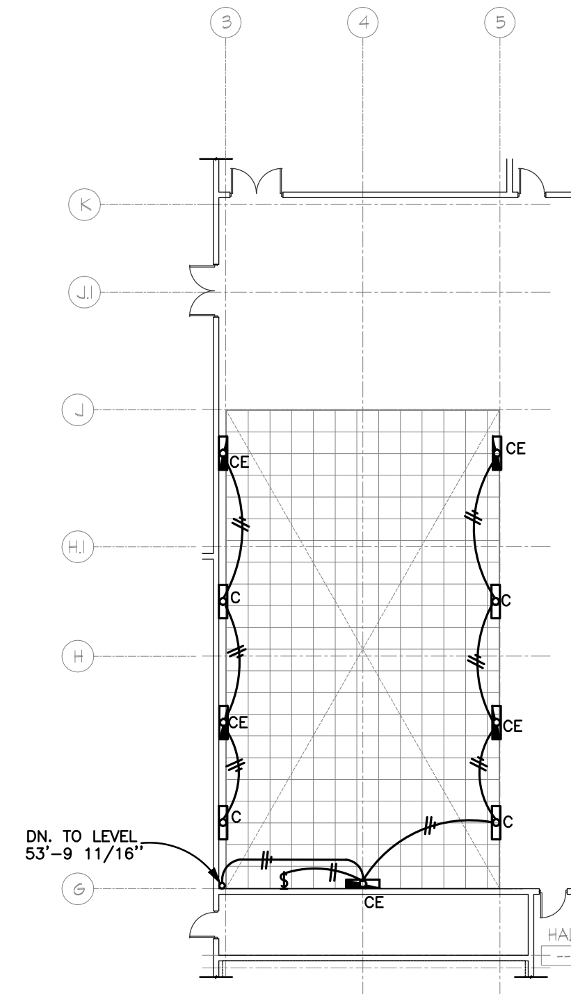
DRYER AREA TOWER (LEVEL: 71'-0" 3/16") SCALE: 1/8" = 1'-0"
