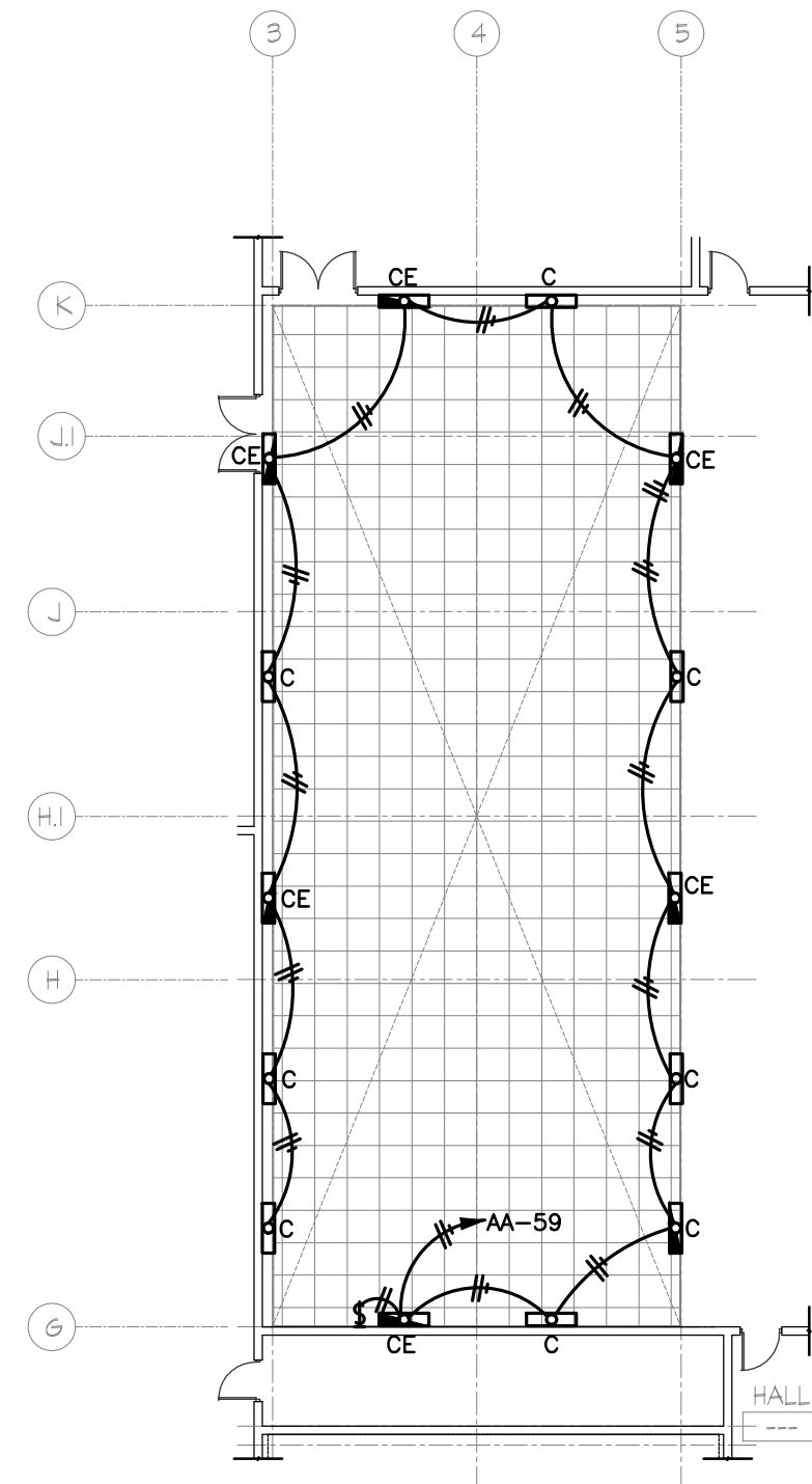
DRYER AREA TOWER (LEVEL: 52'-0" 11/16") SCALE: 1/8" = 1'-0"
