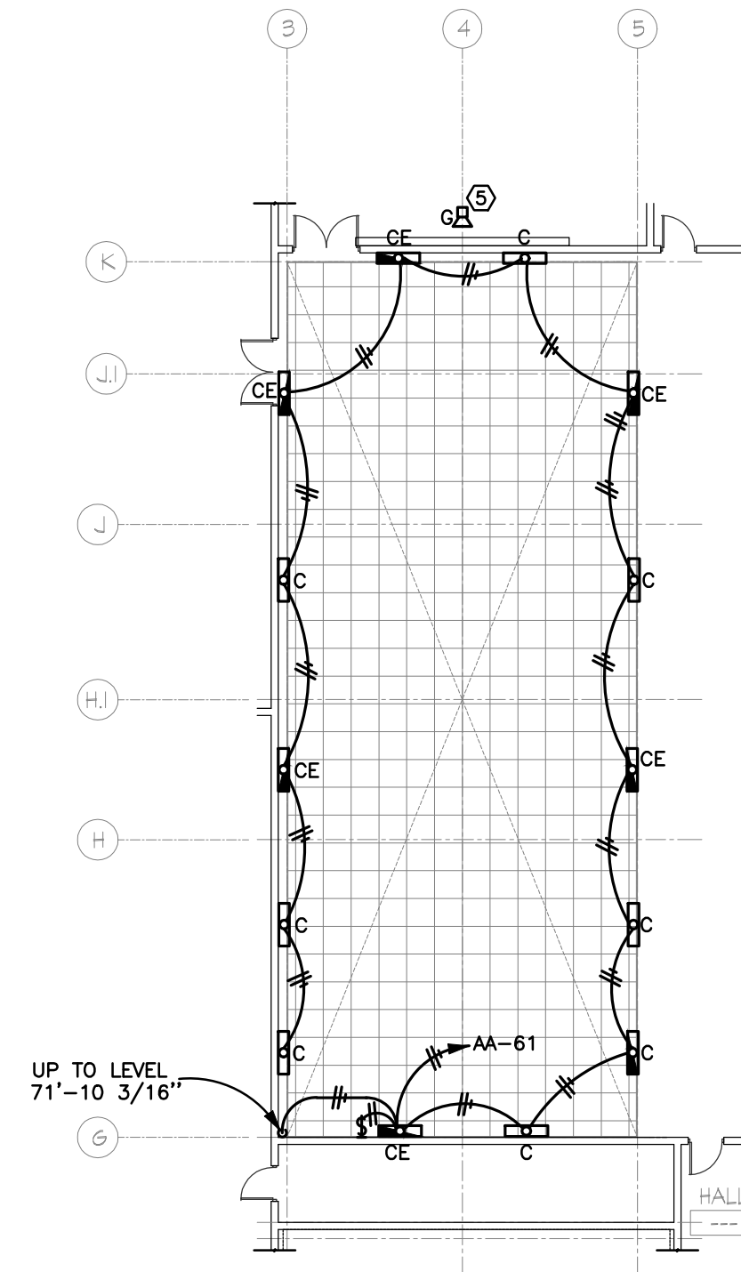
DRYER AREA TOWER (LEVEL: 58'-0" 11/16") SCALE: 1/8" = 1'-0"
